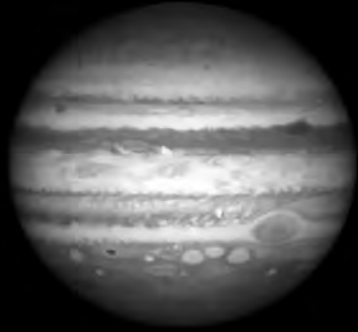
Jupiter 139,822 km
